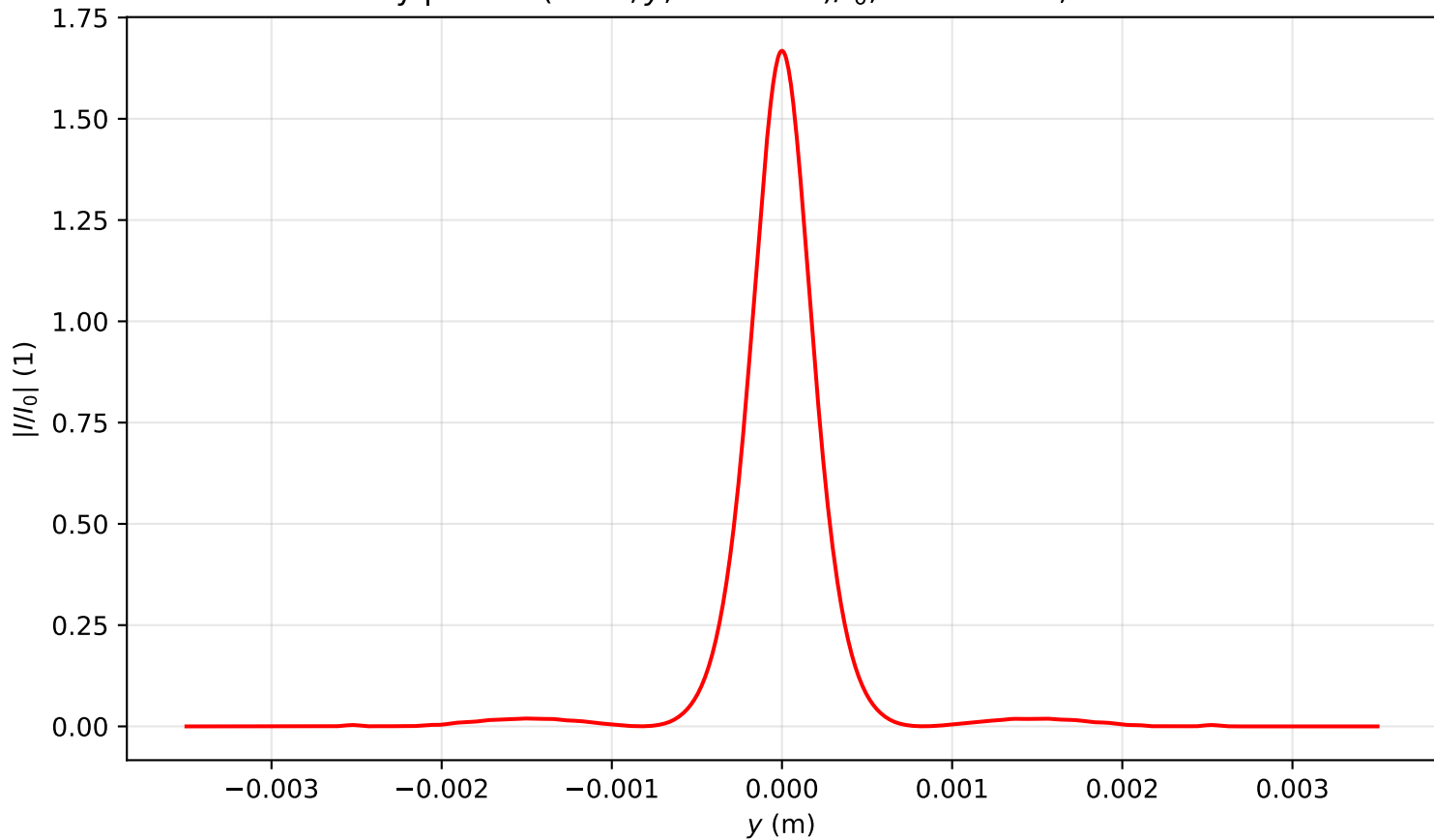
Intensity profile I(x=0, y, z=1.115)/I_0 , P_{in}=1.0P_{cr} , artificial time
